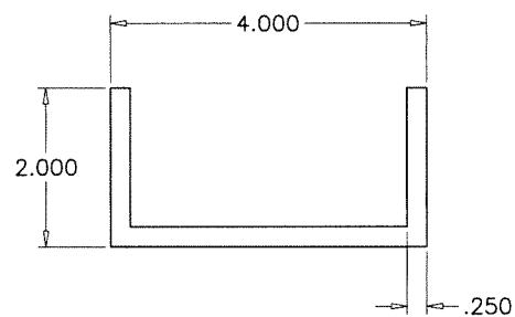
2 BOTTOM CHANNEL
