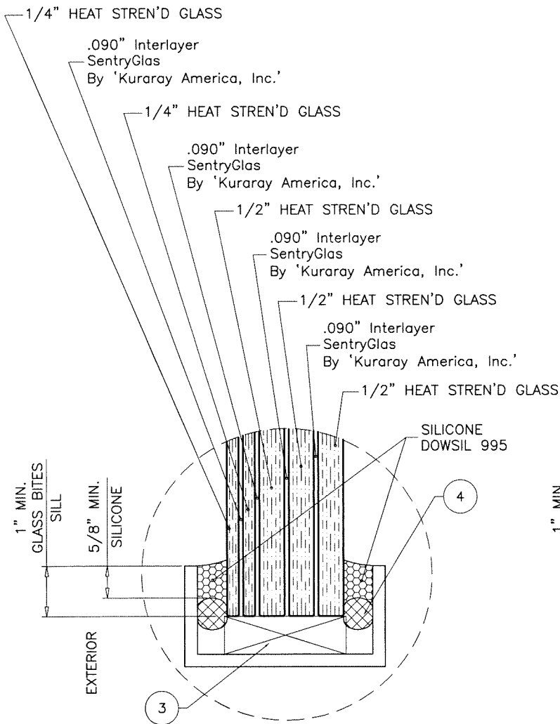
GLAZING DETAIL 2-5/16" OVERALL LAM. GLASS
