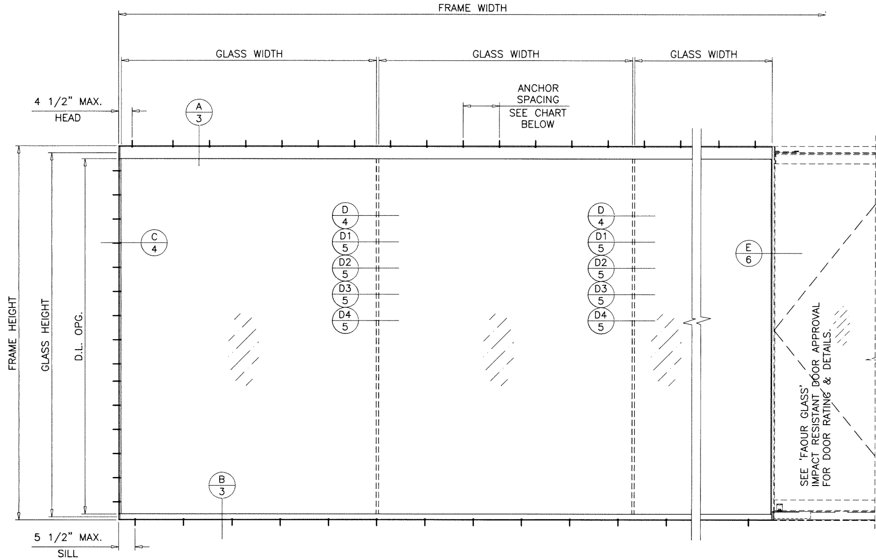
TYPICAL ELEVATIONS
